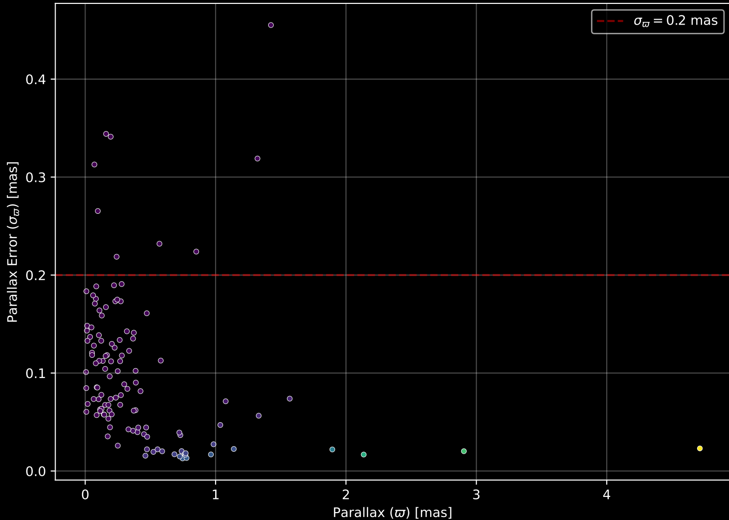
APOGEE DR17 Field: [018+02] Parallax Quality (n= 119)
