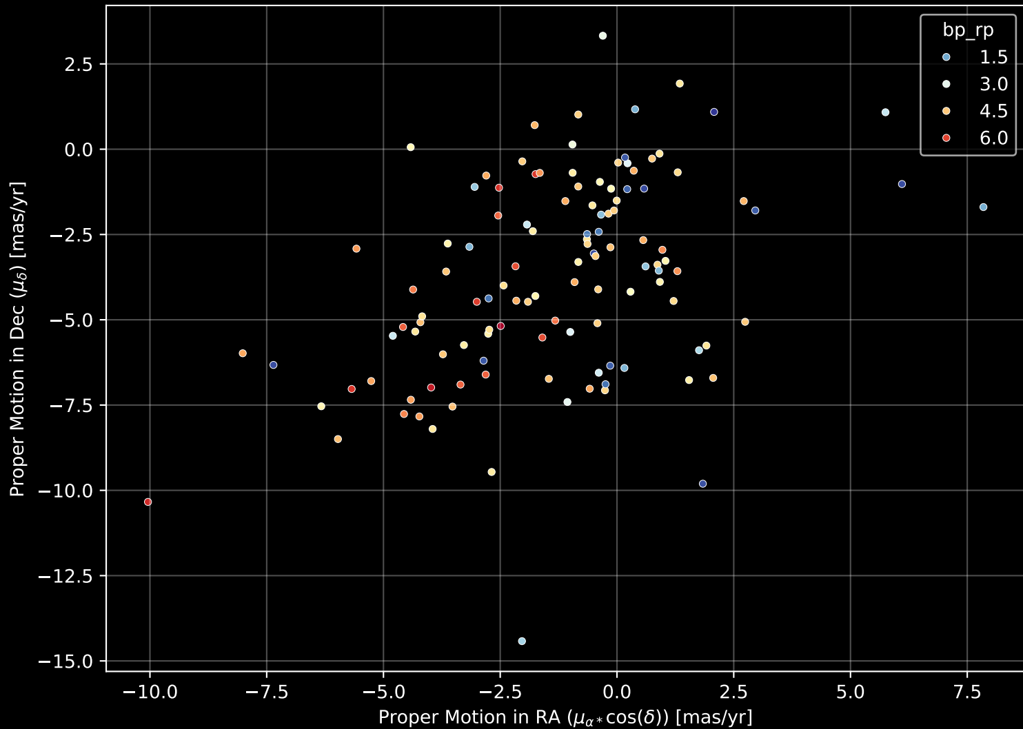
APOGEE DR17 Field: [018+02] Proper Motion Diagram (n= 119)
