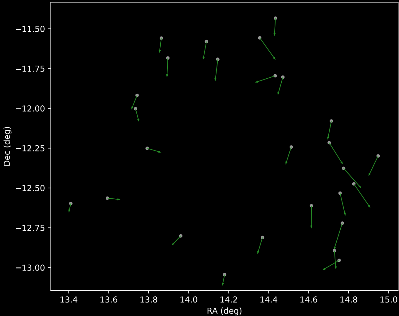
APOGEE DR17 Cluster 4 Proper Motion Vectors (n=27)
