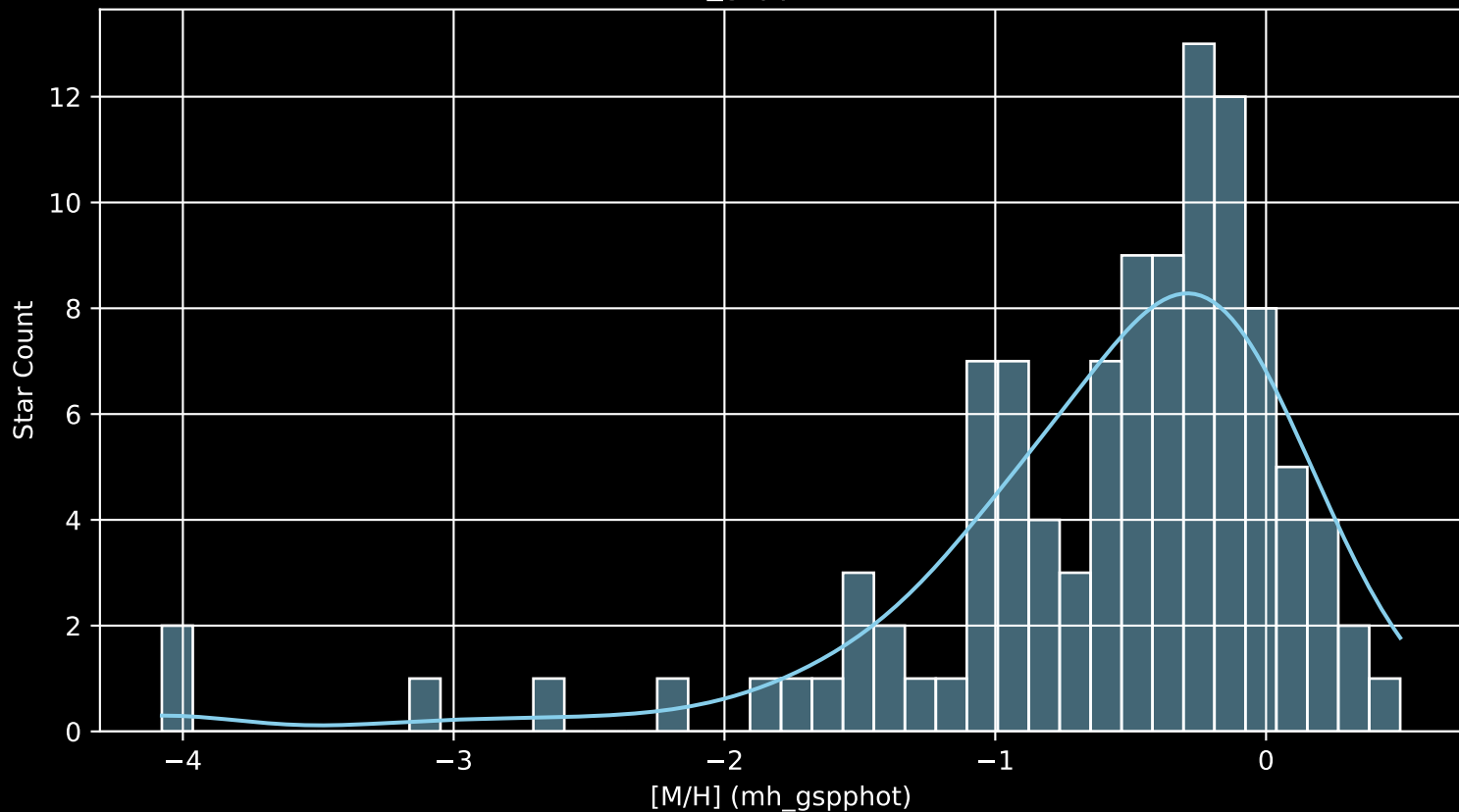
APOGEE DR17 Field: [018+02 [M/H] (mh_gspphot) (n= 106)
