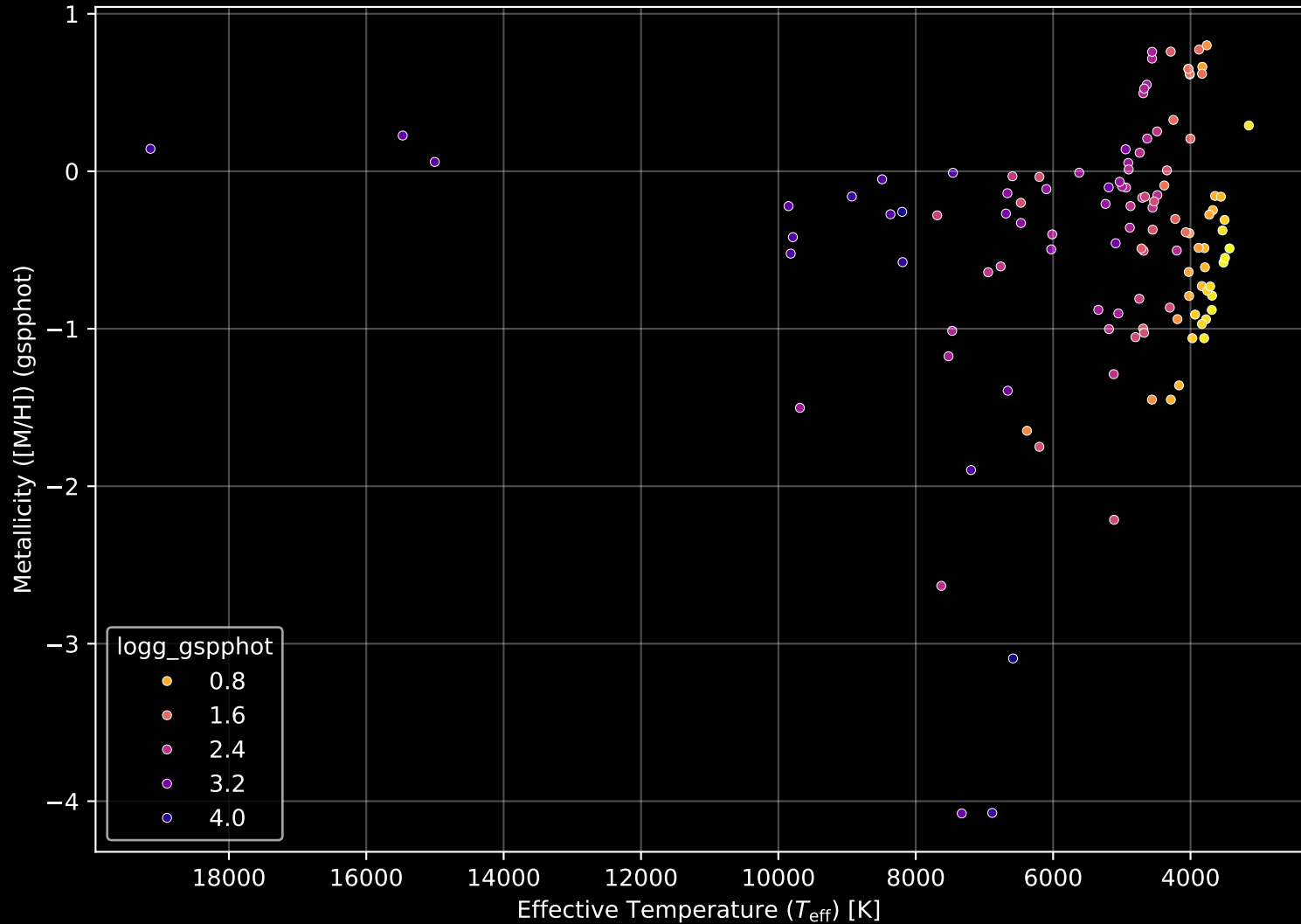
APOGEE DR17 Field: [018+02] Stellar Population Parameters (n= 119)
