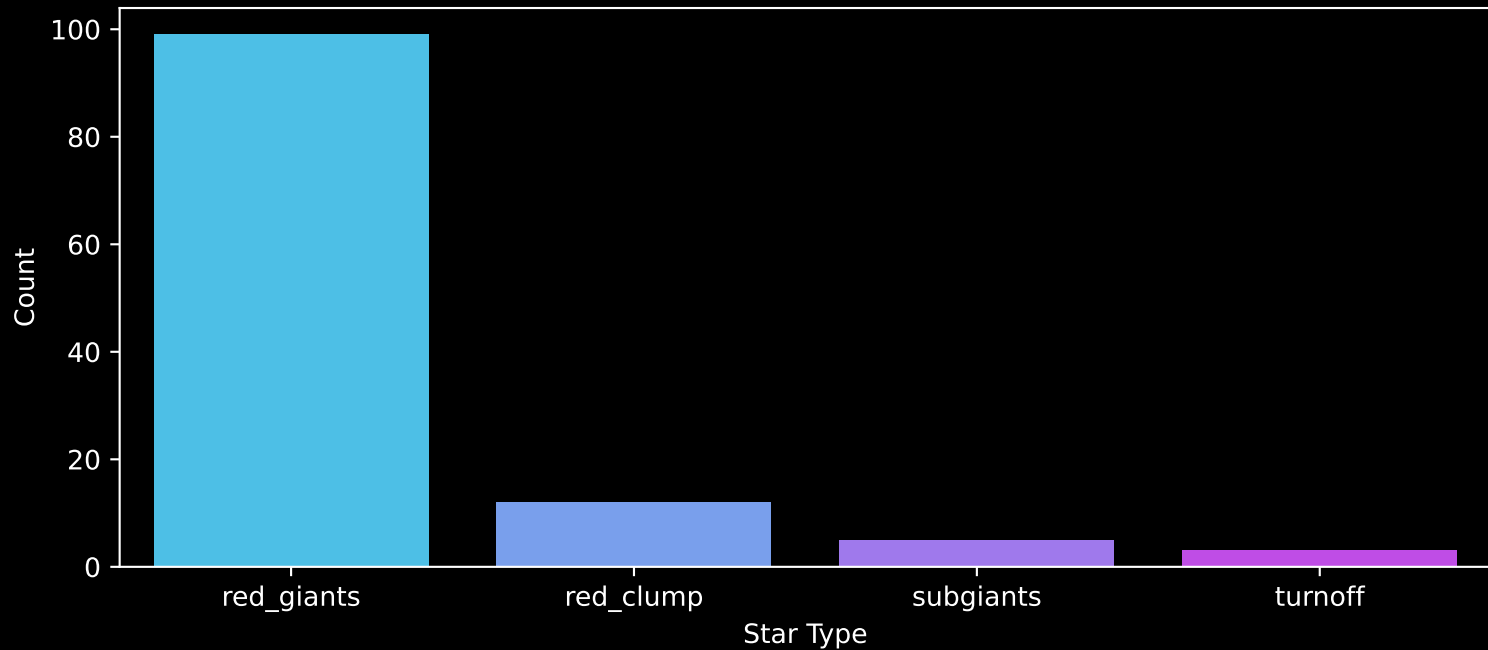
APOGEE DR17 Field: [018+02] Count plot of Star Type
