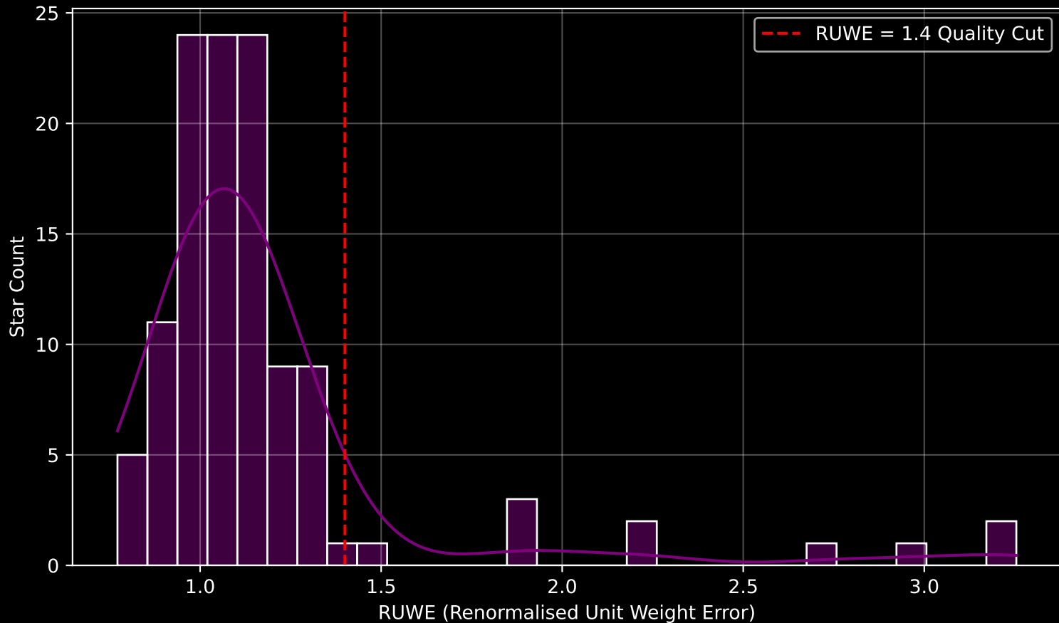
GAPOGEE DR17 Field [018+02] RUWE Distribution (n= 117)
